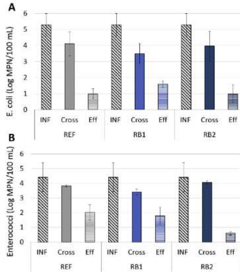
Fig. 5. Concentrations (Log MPN/100 ml) of E. coli (A), and Enterococci (B) measured at inflow (INF), Crosswise piezometer (Cross) and effluent (Eff) samples from REF, RB1, and RB2 systems.
