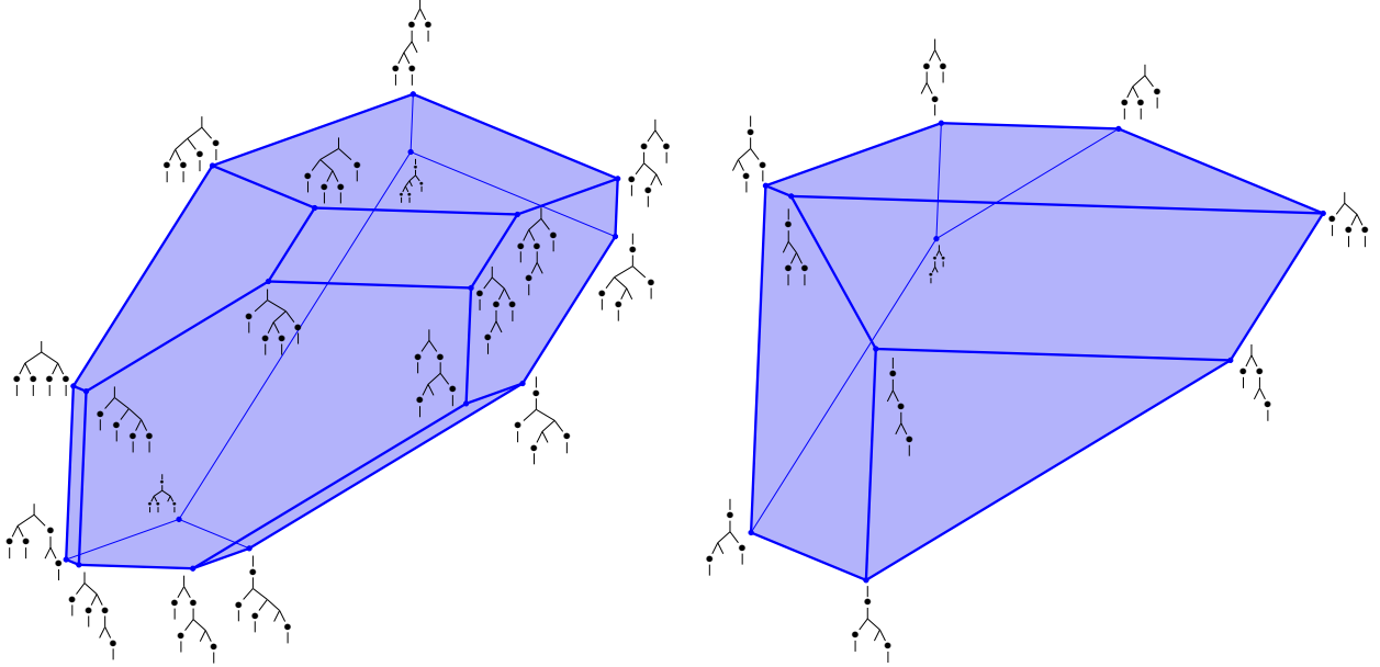
FIGURE 14. The \alpha -associpahedra for \alpha = \text{OIOI} (left) and \alpha = \text{OOOI} (right), realized as faces of the pebble tree polytopes \text{PTP}_4^{1,0} and \text{PTP}_3^{1,0} .
