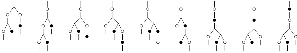
FIGURE 10. A sequence of flips in maximal ○-balanced and ●-unbalanced \{\circ, \bullet\} -pebble trees.
