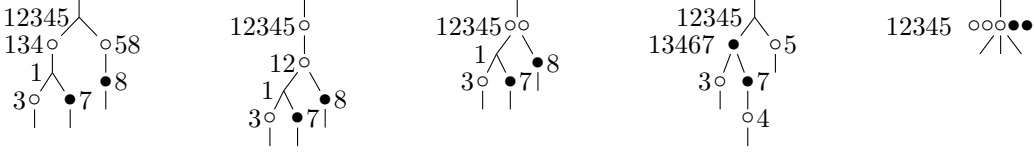
FIGURE 7. Some \circ -balanced and \bullet -unbalanced \{\circ, \bullet\} -pebble trees T and the associated simplicies \Lambda(T) . Each node n of T is labeled by the concatenation of the elements of the set \lambda(T_n) .
