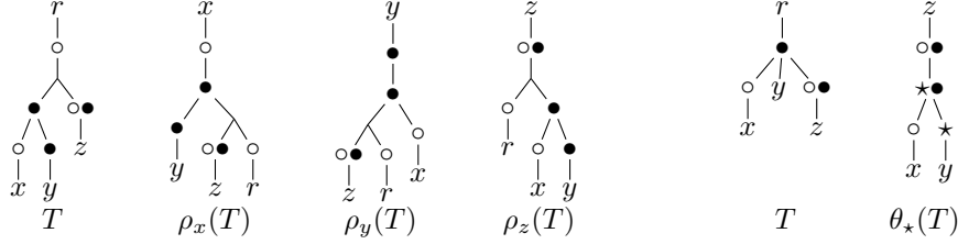
FIGURE 3. A fully balanced \{o, \bullet\} -pebble tree and the fully balanced \{o, \bullet\} -pebble trees obtained by rerooting it at leaves x , y and z respectively (left). A fully unbalanced \{o, \bullet\} -pebble tree and the fully balanced \{o, \bullet, \star\} -pebble tree obtained by \star -uprooting it (right).
